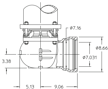
6-INCH TYTON ® JOINT CONNECTION
