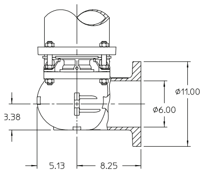
6-INCH CLASS 125 ANSI FLANGED CONNECTION
