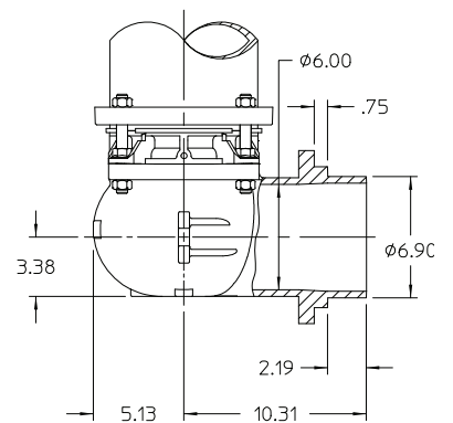
6-INCH PLAIN END W/INTEGRAL MJ GLAND CONNECTION
