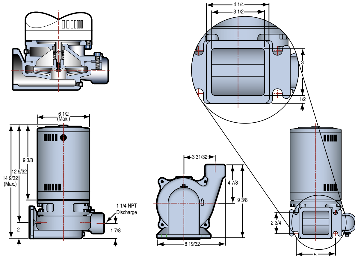
D51DM (1 1/4 X Flange X 5) Vertical Flange Mounted See Diagram for Dimensions in Inches
