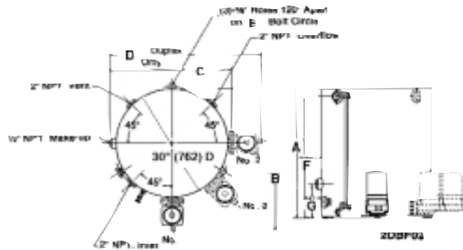
RECEIVER DIMENSIONS
