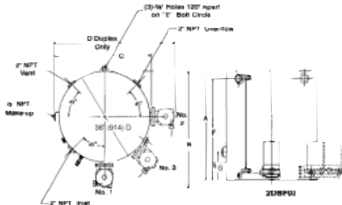
RECEIVER DIMENSIONS
