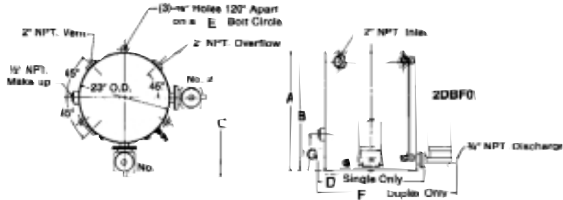
RECEIVER DIMENSIONS
