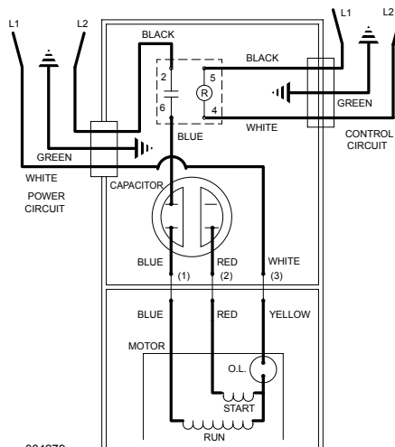
004279 WIRING DIAGRAM FOR MODELS XE4405 ALL REVISIONS
