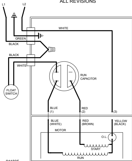
011835 WIRING DIAGRAM FOR MODELS WD4405 ALL REVISIONS
