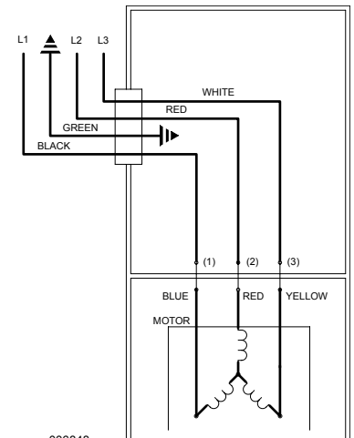
006848 WIRING DIAGRAM FOR MODELS J4405, F4405, G4405 AND BA4405 ALL REVISIONS
