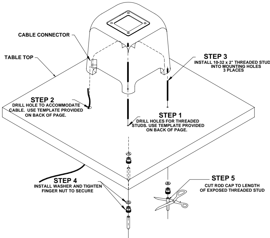
Standard SAS-SM8 mounting using SAS-MK mounting kit.
