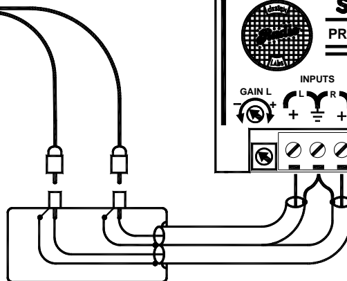
RDL ACB-2 (OPTIONAL)
