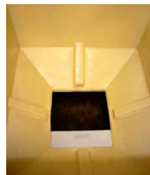
CM-52 from inside - hopper gate partially open. Hopper opening measures 20" x 16".
