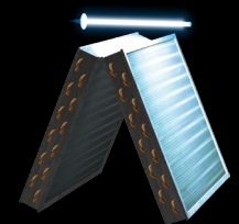
'A' Coil Perpendicular Mounting
