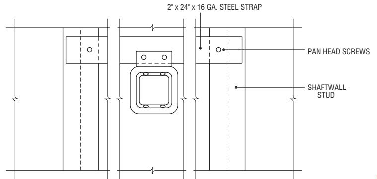
ELECTRICAL OUTLET SUPPORT 09260W Scale: 3" = 1'-0"
