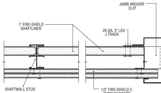
SHAFTWALL 7'-0" ELEVATOR DOOR JAMB (Section A-A)
