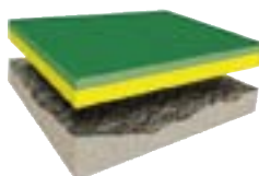
Standard vinyl floorcovering on uneven subfloor
