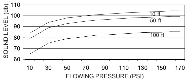
TYPICAL DECIBEL SOUND LEVELS - WM, WM-2
