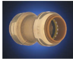
Coupling CxC 1/2", 3/4" & 1"
