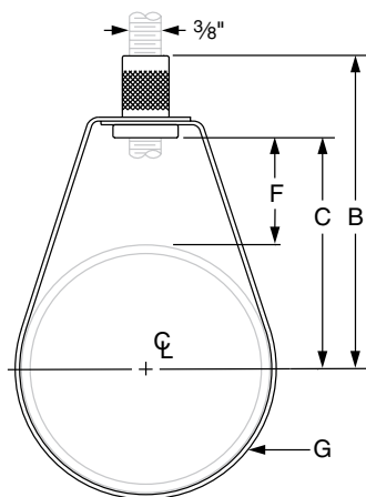
1 1/2" through 4" pipe
