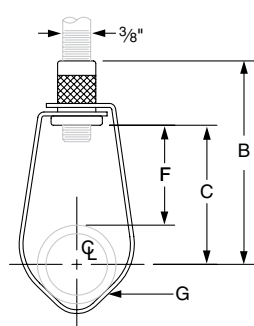
1/2" through 1 1/4" pipe
