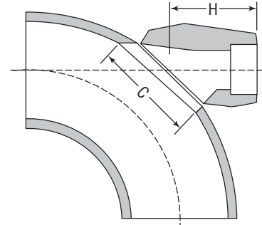
SOCKET-WELD
