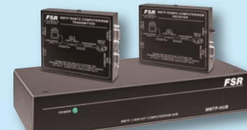
TWISTER-MMTP Hub, Transmitter and Receiver Computer Video over CAT-5 (800')
