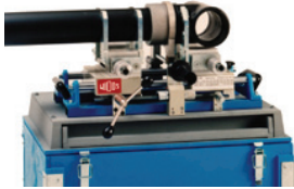
Shop 4 - For socket fusion welding of components from 20 - 110mm (1/2" - 4").
