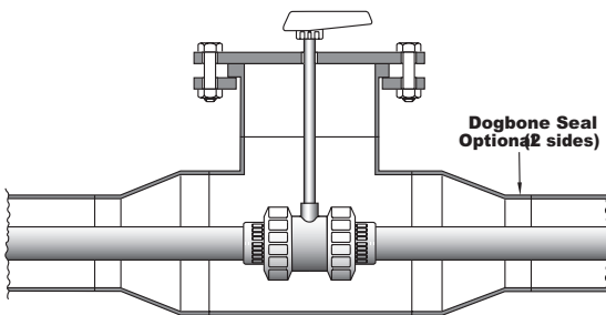
Figure G-14. Double contained ball valve with stem
