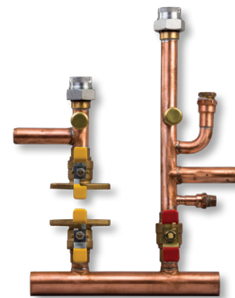
NHB Primary Manifold Kit GFFM-MSOZUS-001
