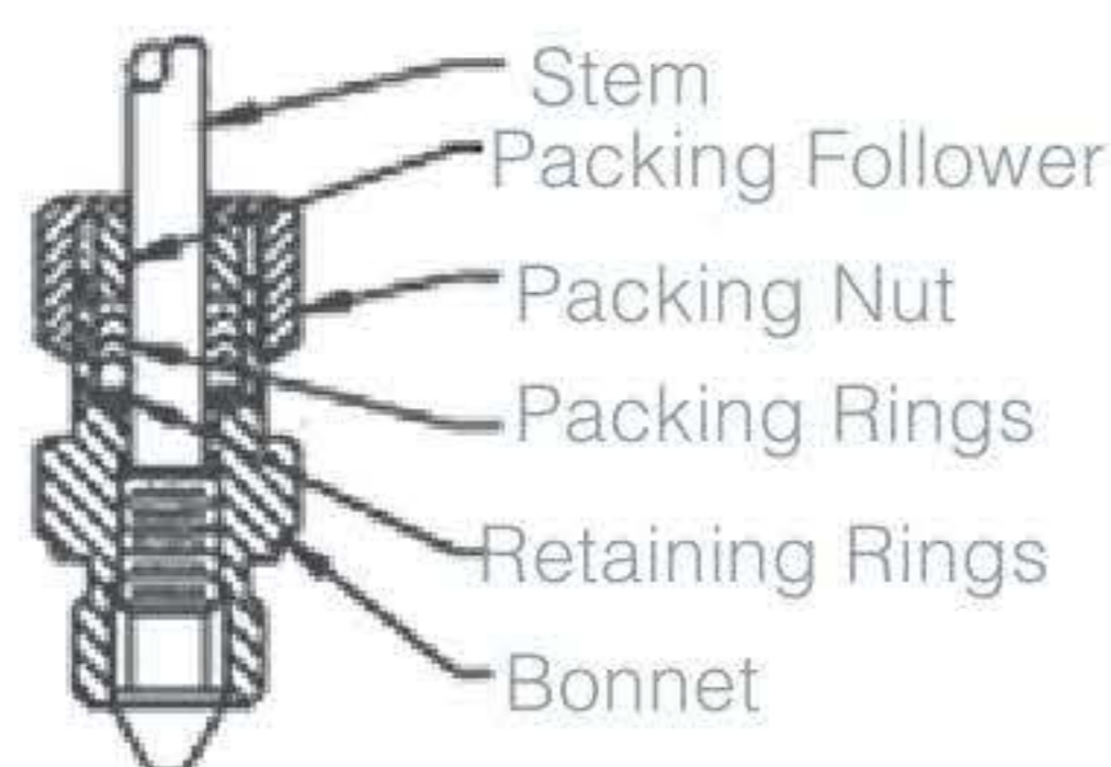
Bonnet Detail
