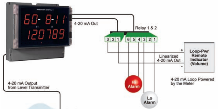
Round Horizontal Tank Signal Input Conditioner
