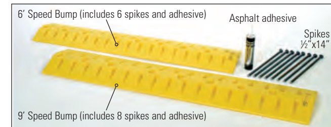
Model 1792 6' Speed Bump - Cable Guard 10" w x 2" h x 72" l Inside Channel Dimensions: 1.25" w x 0.875" h
