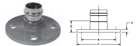
PC741 ⚠️ Companion Flange P x Flange - Cast Bronze Flange/ Wrot Outlet
