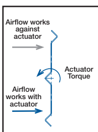
Balanced Blade Requires Less Torque
