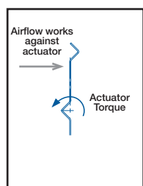
Unbalanced Blade Requires Higher Torque
