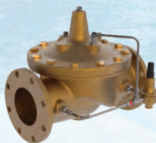
90-42 Seawater Service Pressure Reducing Valve
