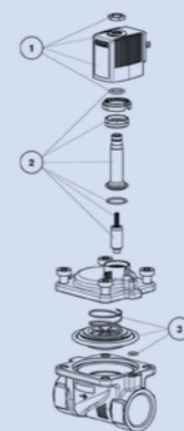
WW A – Normally closed
