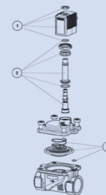
WW B – Normally open
