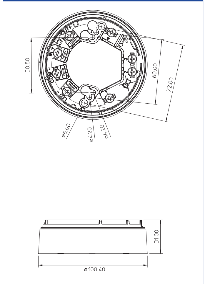
Orbis Marine Relay Base dimensions
