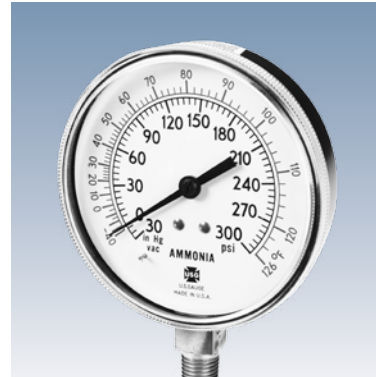
Model 1706 Ammonia Refrigerant Gauge: Ammonia compressor and refrigerant system specific • Silicone dampened movement extends gauge life • Pressure/Temperature scale dial
