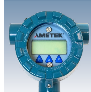
Model DT-8300 EX Explosion Proof Digital Thermometer: FM approved Explosion Proof • NEMA 4x housing • Battery powered or line powered
