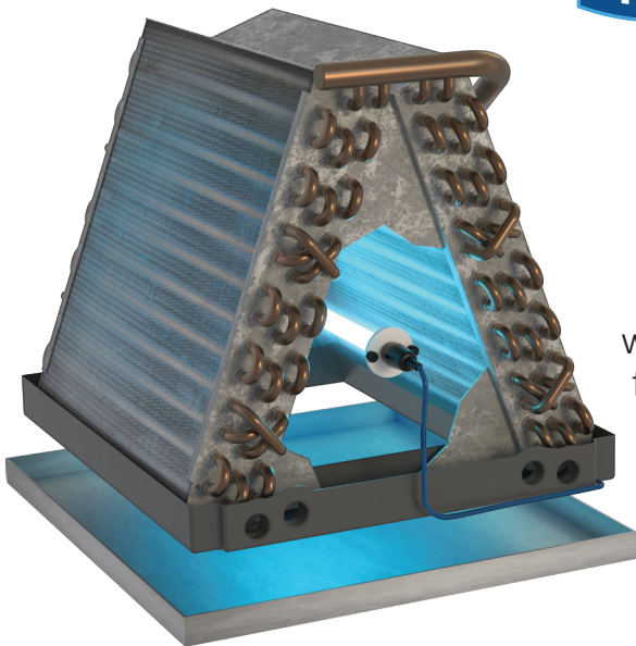
HVAC cooling coil with Fresh-Aire UV® light
