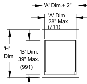
Typical Style CO and WO Construction
