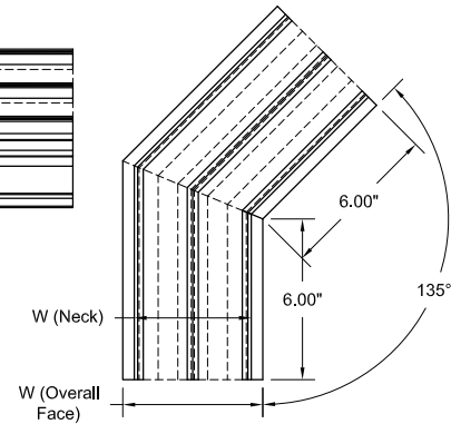
Mitered Corner 135° - Top View
