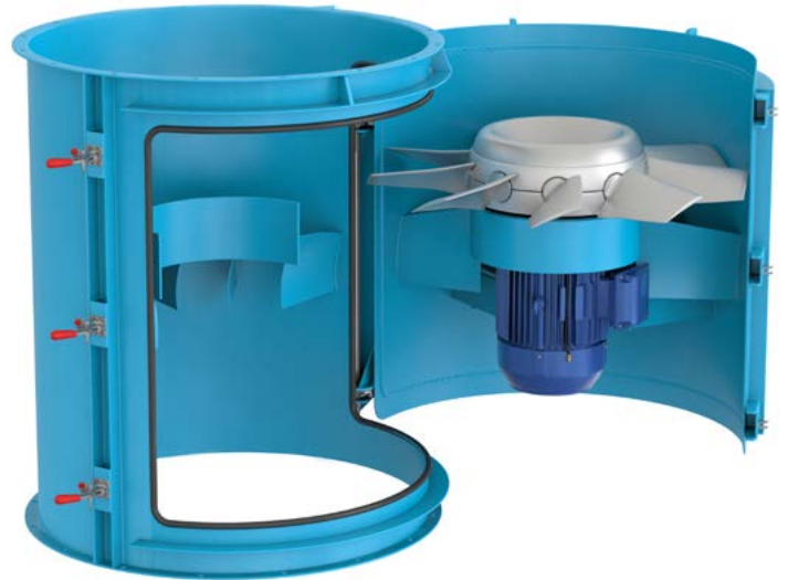
Swingout Construction
