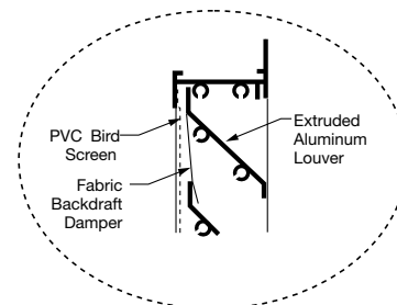
Louver Cutaway
