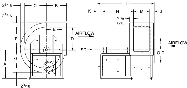
D & M are inside dimensions.
