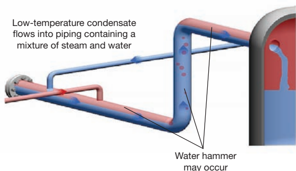
▲ Figure 16. Water hammer may be generated by different steam or flash steam sources, far from or upstream of the convergence point of transport piping. In such cases, pinpointing the cause can be challenging, but it is always wise to first check for leaking traps or open bypass lines.
