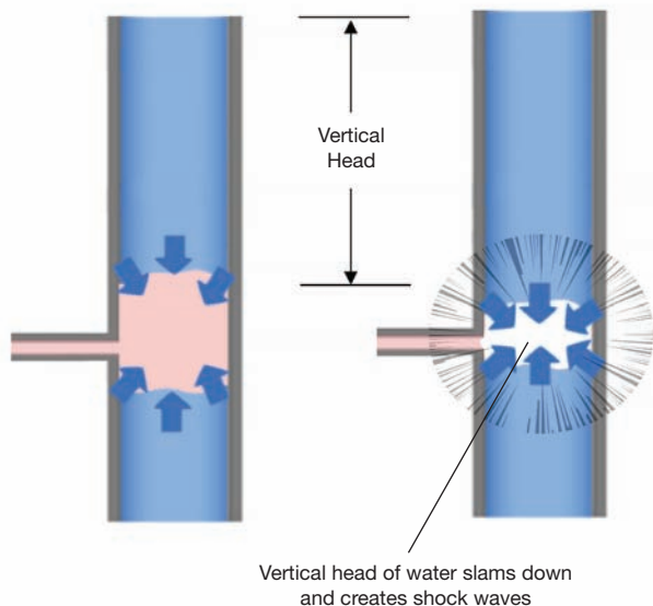
▲ Figure 13. Water hammer can be worse in vertical pipes than in horizontal piping. A vertical head of water above the steam pocket can exert additional pressure on the pocket, and, when the pocket collapses, the accelerating mass of the column of water can exacerbate the shock waves.
