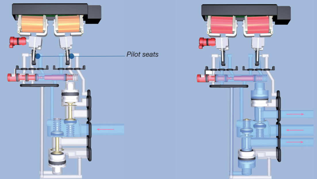
De-energized
