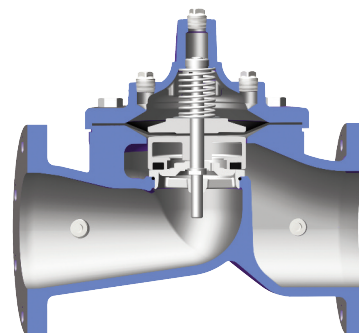
100-20 Hytrol Main Valve - Reduced Port
