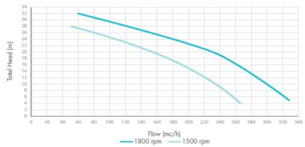
Performance curves 6"
