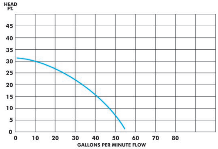
SS233 Performance Curve 2" Discharge
