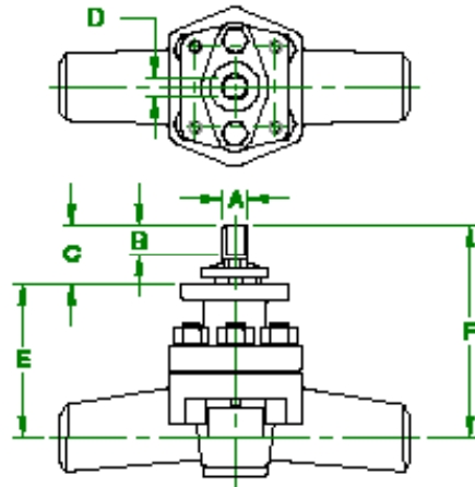
CLASS 600 BUTT WELD STANDARD PORT - SIZE 1 1/2" THRU 2"
