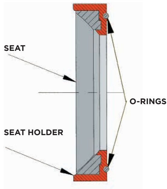
FIGURE 3 SEAT DESIGN 3
