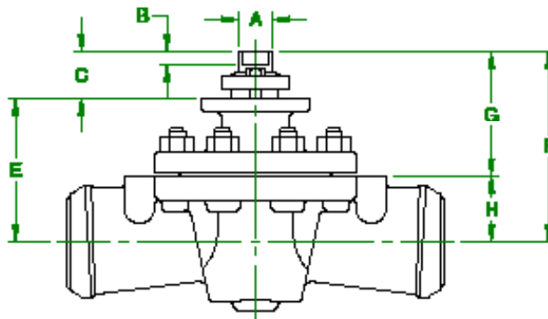
CLASS 600 BUTT WELD STANDARD PORT - SIZE 2" THRU 6"
