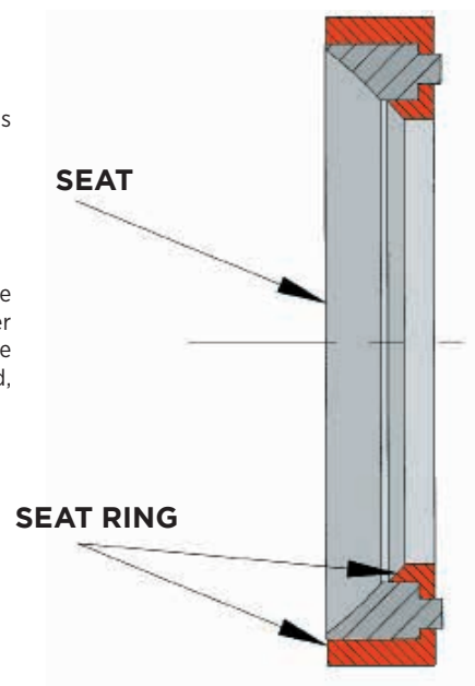
FIGURE 2 SEAT DESIGN 2
