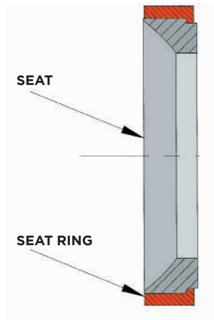
FIGURE 1 SEAT DESIGN 1
