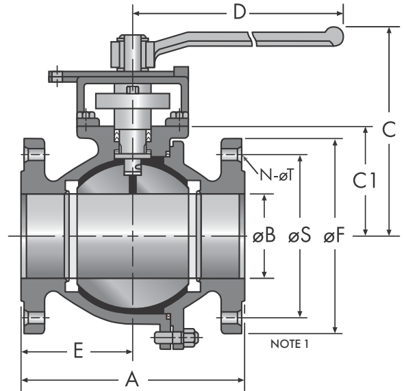
DIMENSIONS – Secure Mount
