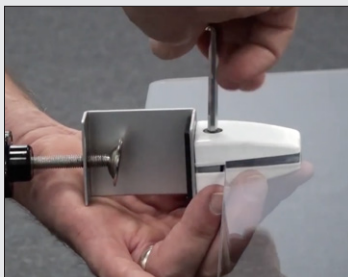
Step 1 - Attach large clamp with hex wrench
