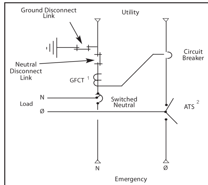
One line diagram of a typical service entrance rated transfer switch. It's available with solid, switched or overlapping neutral poles.
