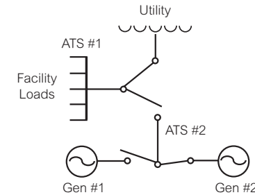
One line diagram of a typical three source power design. The three source transfer switch (ATS #2) automatically connects to the power source that achieves acceptable voltage and frequency first.
