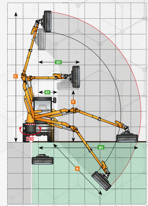
WORK WITH LEFT BOOM
