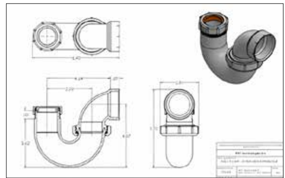
Dimensional Drawings
