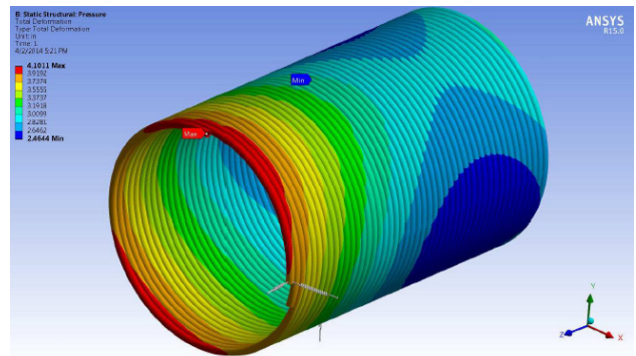
▶ Fulton coils are designed for the process and subjected to stress and temperature analysis to ensure longevity in the field.
